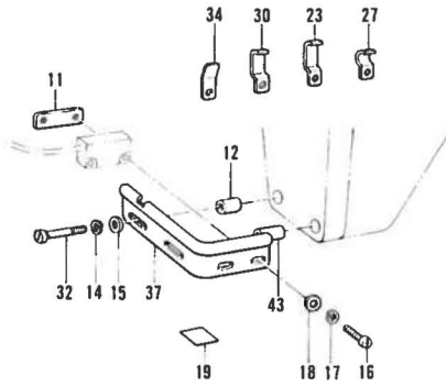
Sensor #1-7 #2-7, B774
