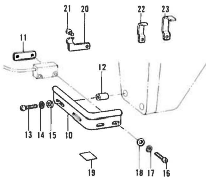
Sensor #1-1,1-2,2-1,2-2,B737,Mark II,748
