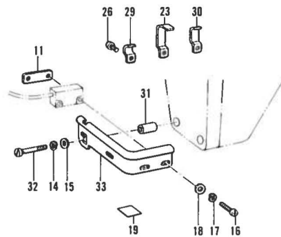
Sensor #1-4,2-4,B791
