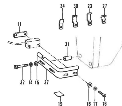
Sensor #1-5,2-5,B793,795
